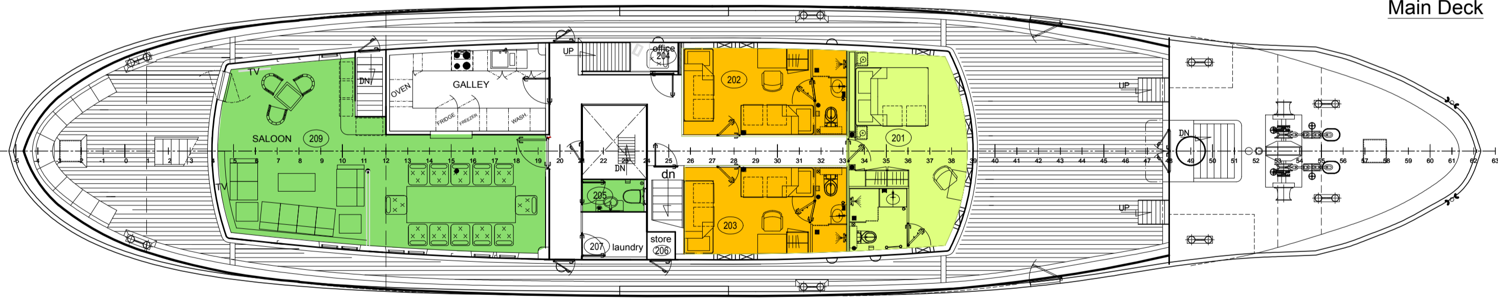
Main Deck
