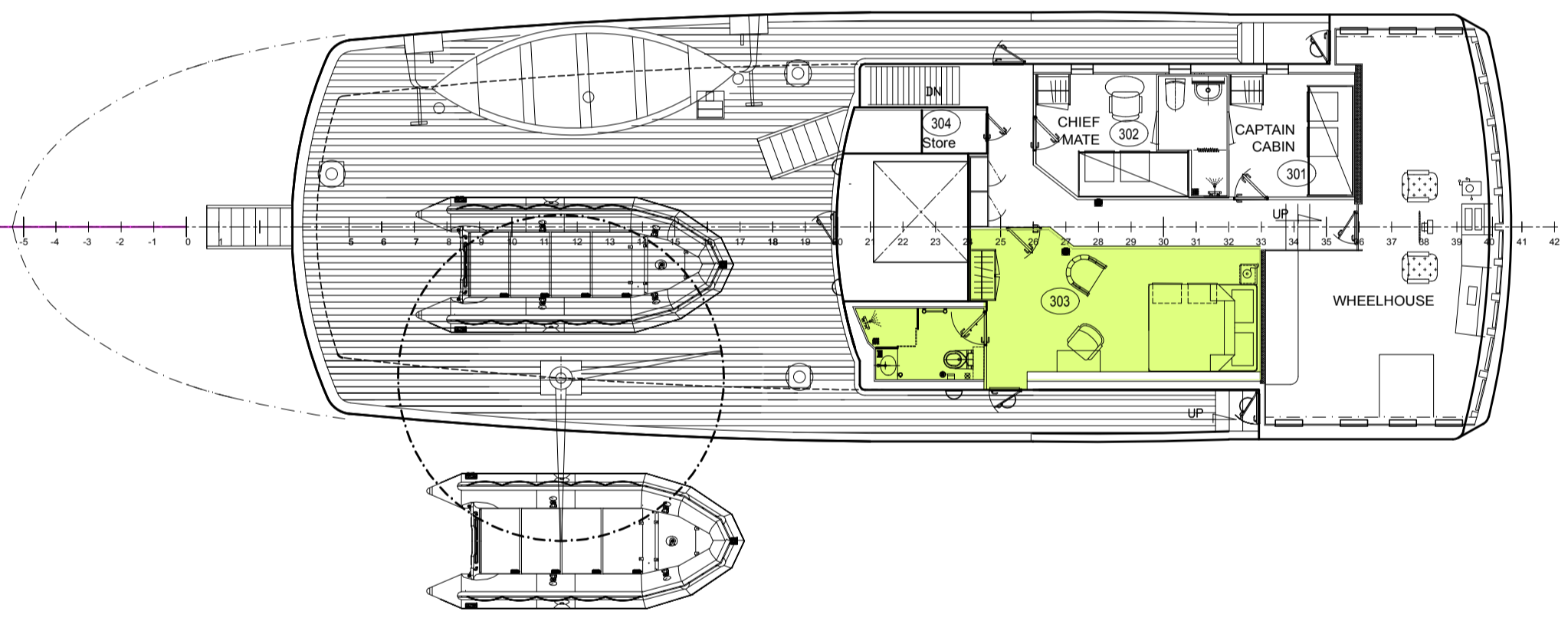
Bridge Deck
